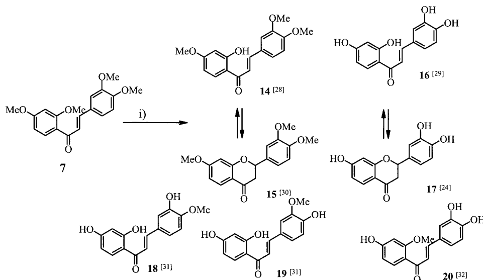
Scheme 2. i) \text{EtONa} , dry DMF, 4 h at reflux
